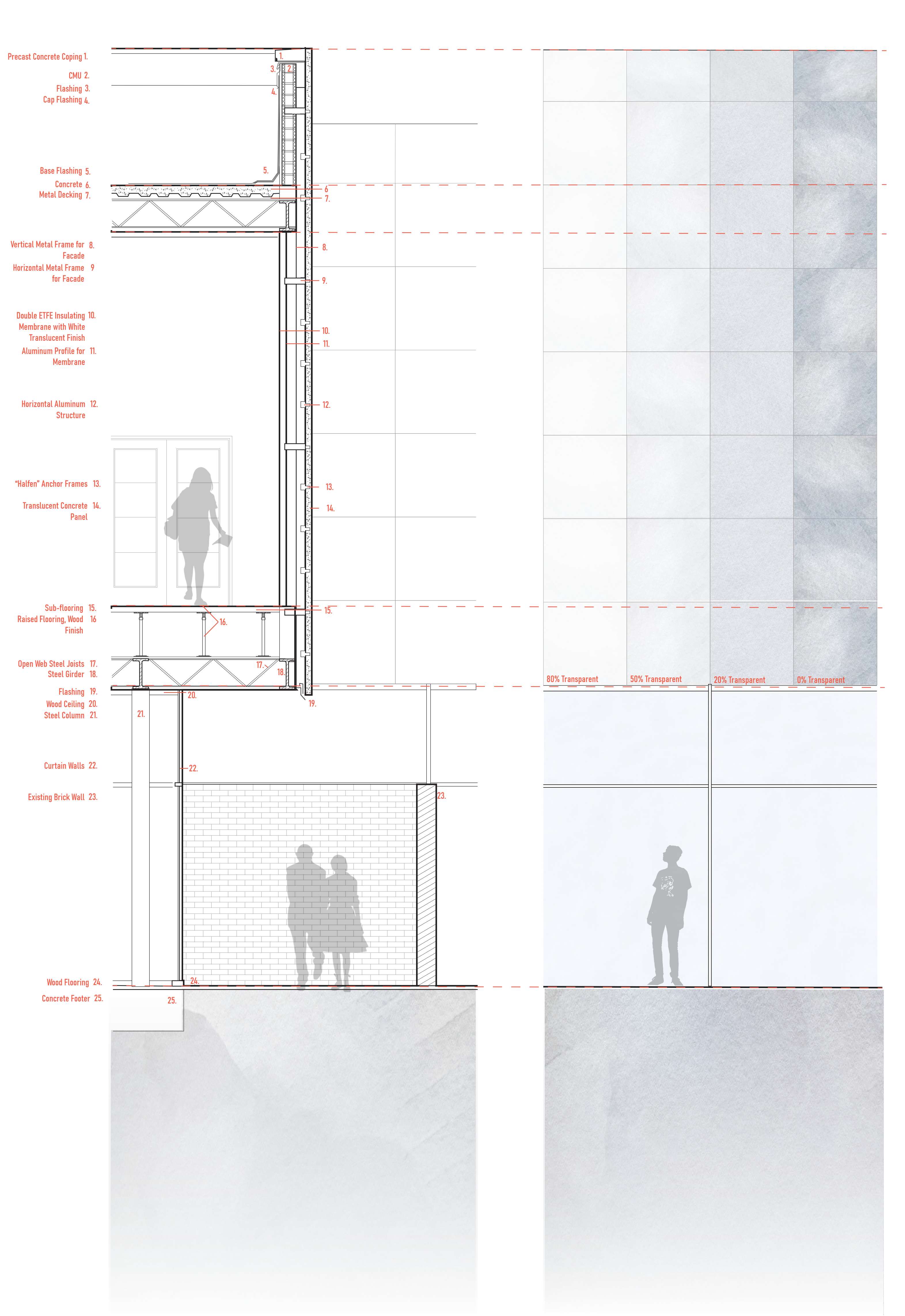
WALL SECTION DETAIL
